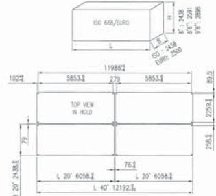
Container Pockets used in Hold
