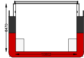
Front view looking aft
